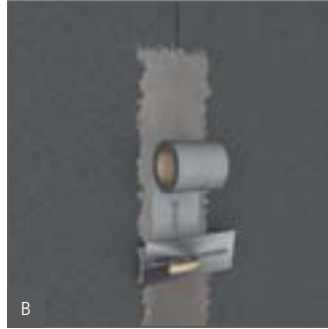
Seal the joints with wedi Tools sealing tape bedded in a layer of Epoxy tile adhesive and quartz sand.
