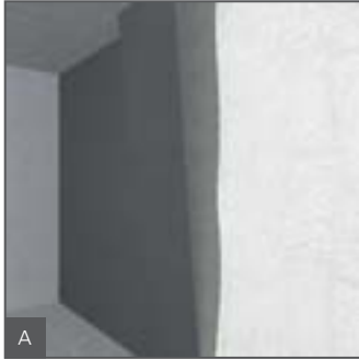
Attach the wedi Vapor building boards across the full surface with tile adhesive.
